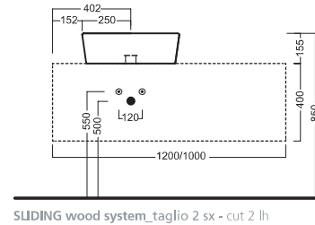
SLIDING wood system_taglio 2 sx - cut 2 lh
