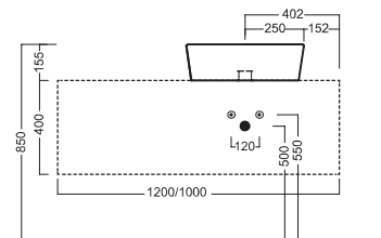
SLIDING wood system_taglio 2 dx - cut 2 rh
