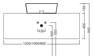
SLIDING wood system_taglio 2 centrale - cut 2 central
