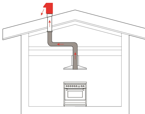
Canopy Install
