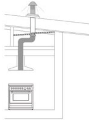
ROOF KITS
