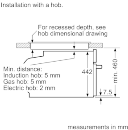
Installation with a hob.
