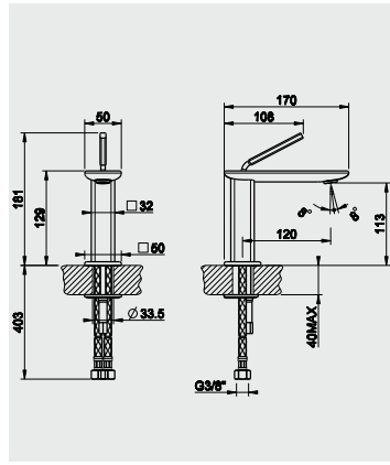
41001 Single lever washbasin mixer without pop-up. 6 Star, 4.5L/min
