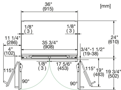
KF2982Vi, KF2982SF, KF2981Vi, KF2981SF, MasterCool, top view, installation drawings
